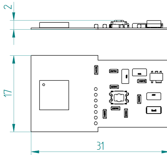
Fig. 1. Dimensions.
